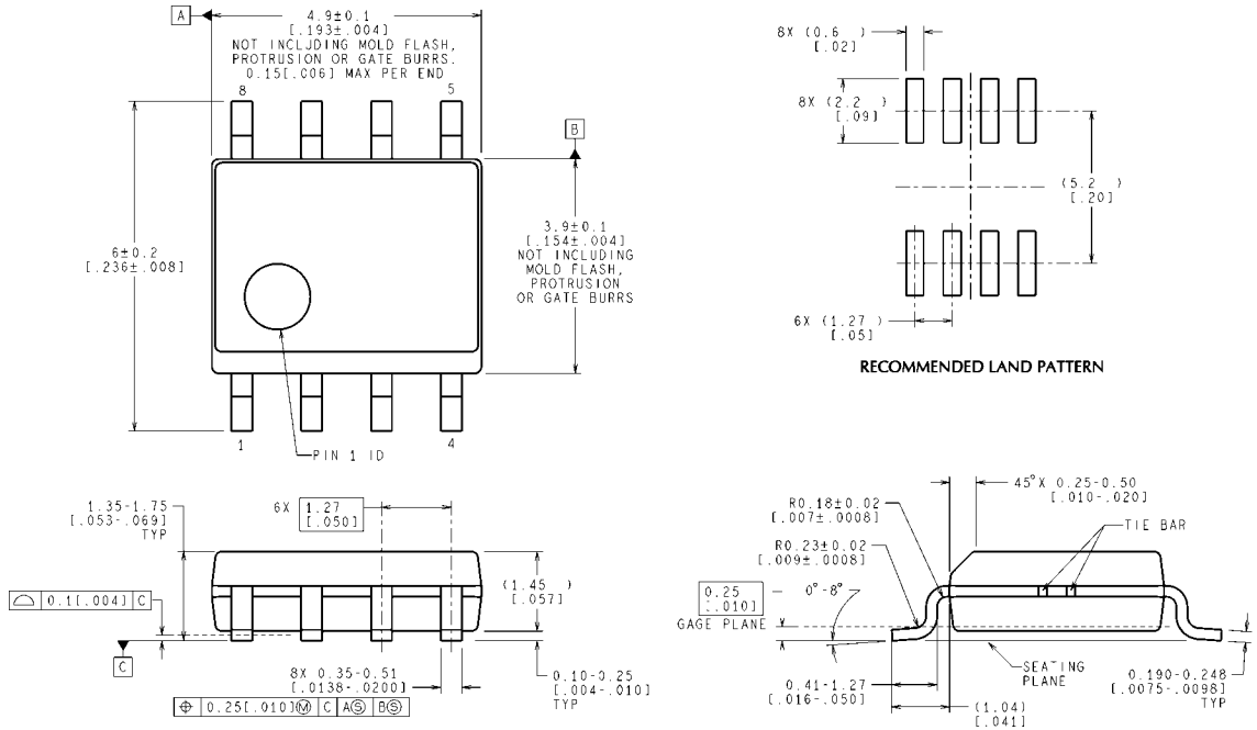
CONTROLLING DIMENSION IS MILLIMETER VALUES IN [ ] ARE INCHES DIMENSIONS IN ( ) FOR REFERENCE ONLY 8-Pin SOIC NS Product Number M08A
